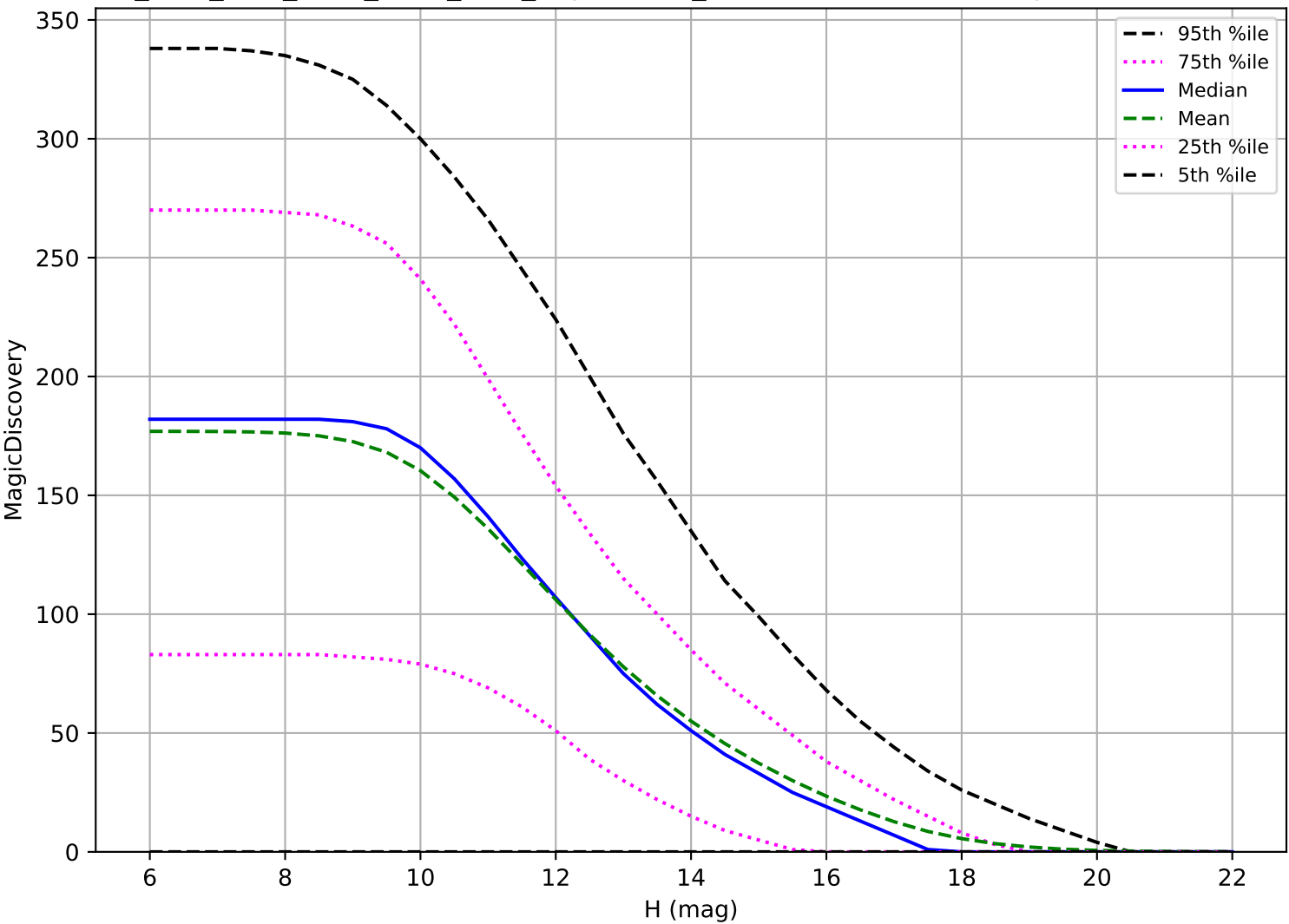
ddf_acor_sf10_lsf20_lsr50_v3.4_10yrs: OCC_r5 6 detections in 60 nights detection loss
