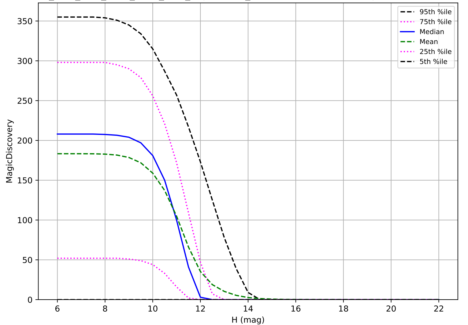
ddf_acor_sf10_lsf20_lsr50_v3.4_10yrs: OCC_r20 6 detections in 60 nights detection loss
