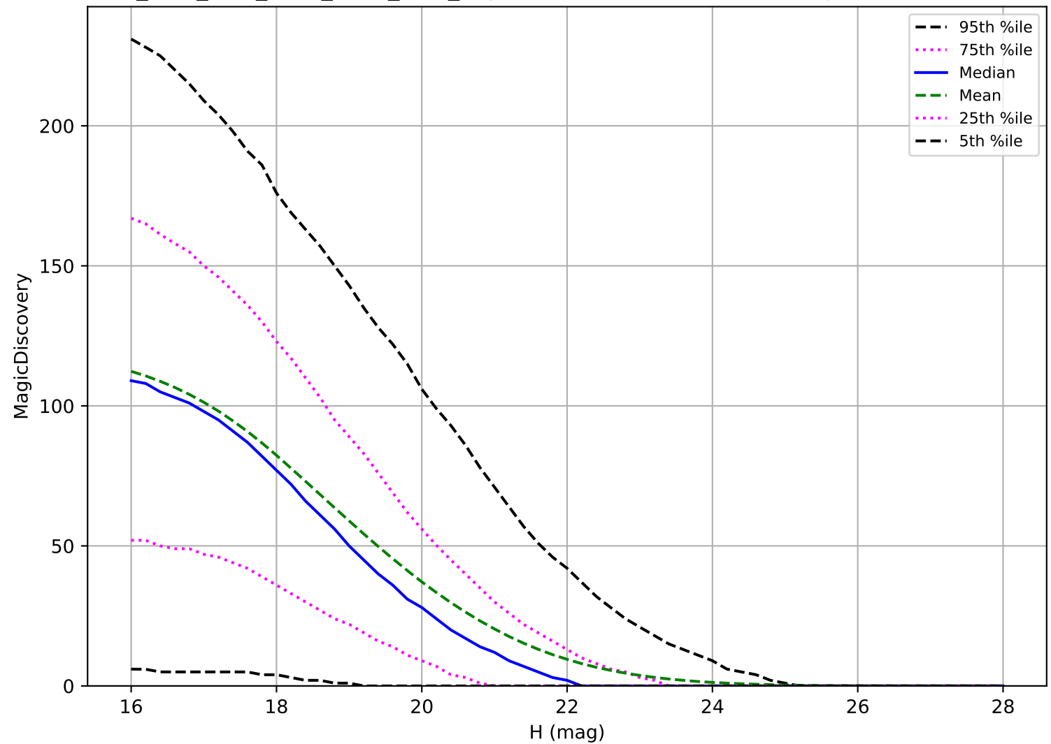
ddf_acor_sf10_lsf20_lsr50_v3.4_10yrs: NEO 6 detections in 60 nights detection loss
