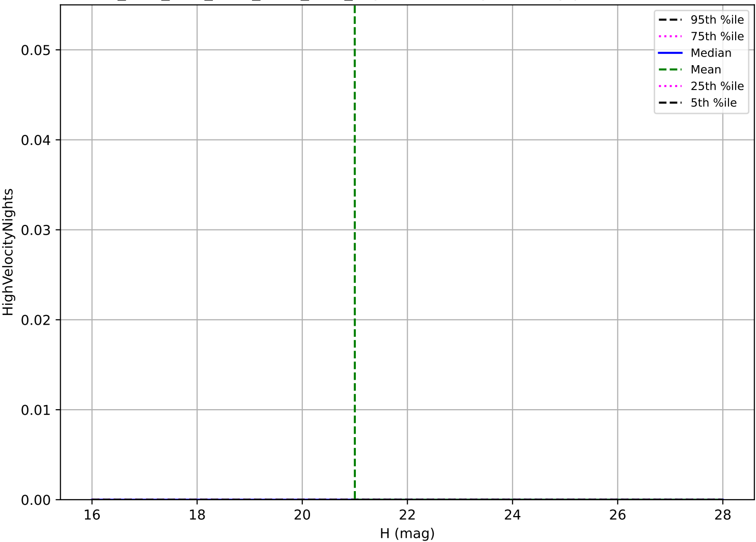
ddf_acor_sf10_lsf20_lsr50_v3.4_10yrs: Vatira High velocity pair detection loss
