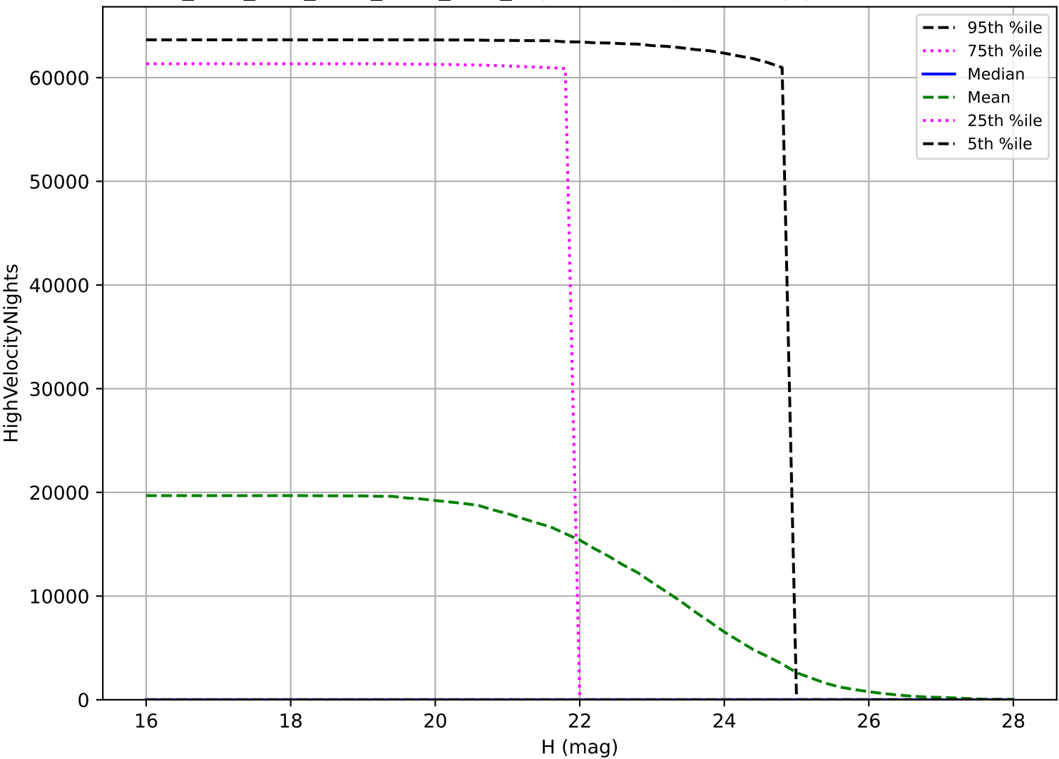
ddf_acor_sf10_lsf20_lsr50_v3.4_10yrs: NEO High velocity pair detection loss
