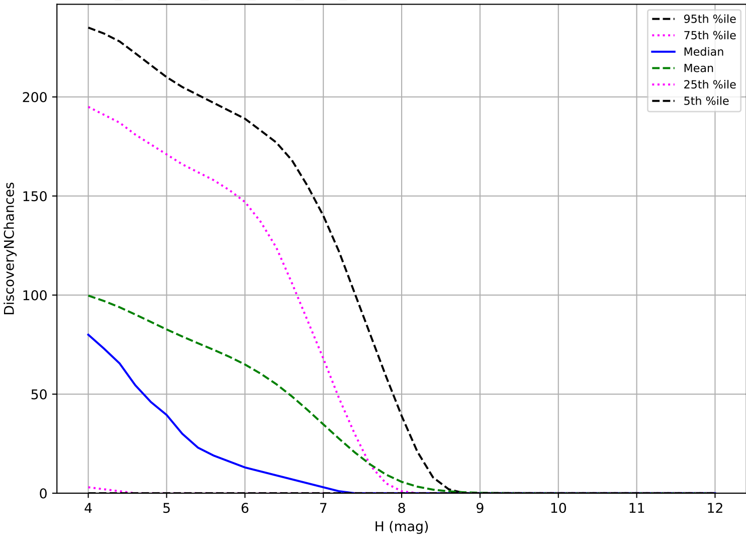
ddf_acor_sf10_lsf20_lsr50_v3.4_10yrs: TNO 3 pairs in 15 nights detection loss
