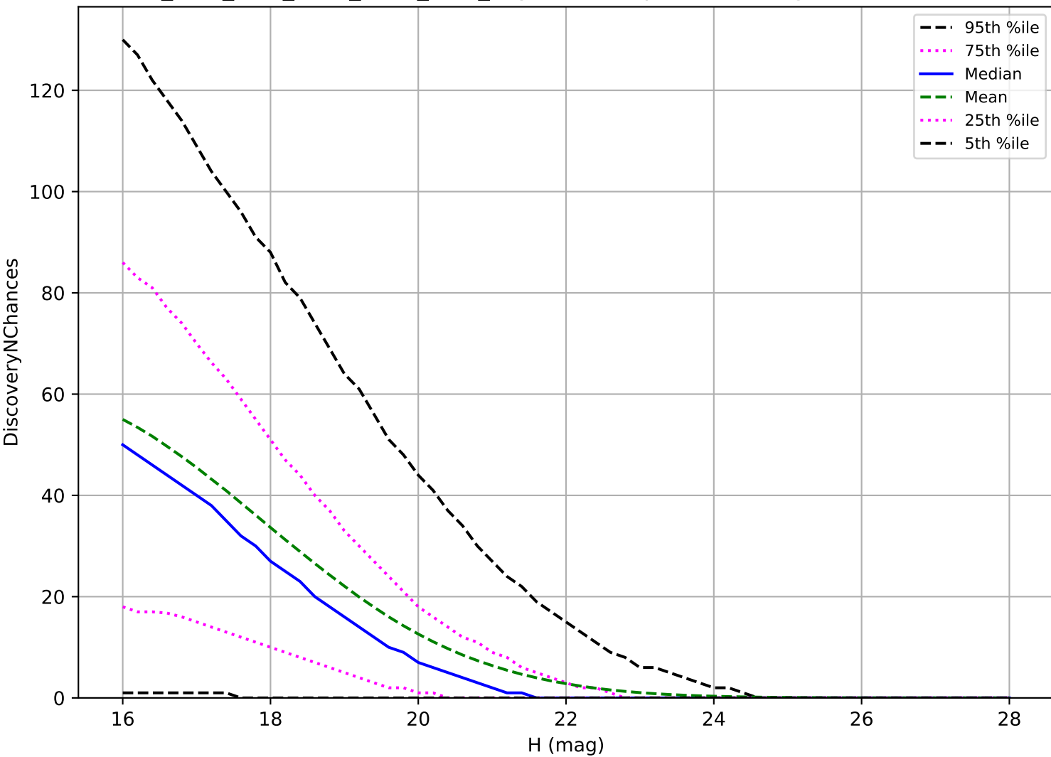
ddf_acor_sf10_lsf20_lsr50_v3.4_10yrs: PHA 3 pairs in 15 nights detection loss
