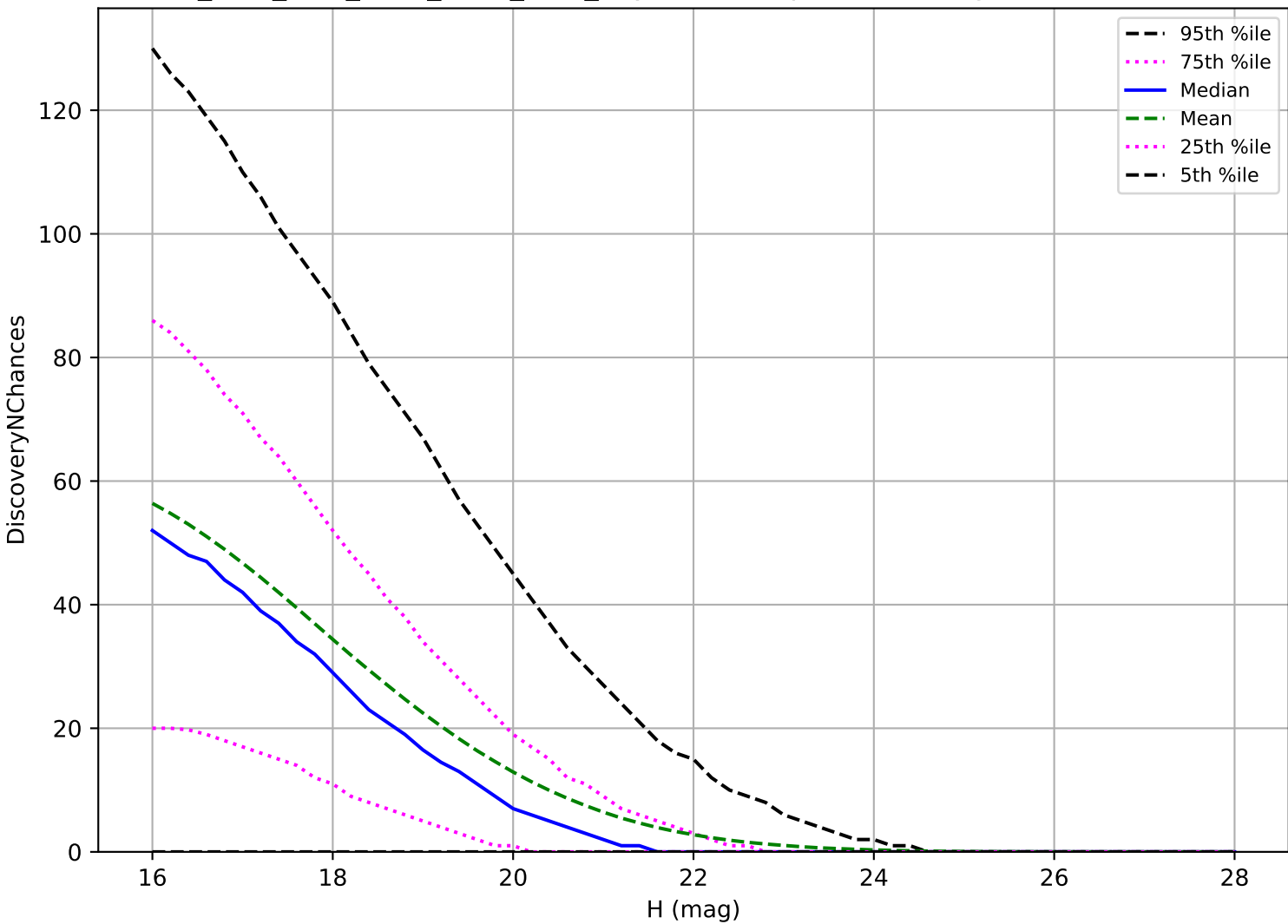
ddf_acor_sf10_lsf20_lsr50_v3.4_10yrs: NEO 3 pairs in 15 nights detection loss
