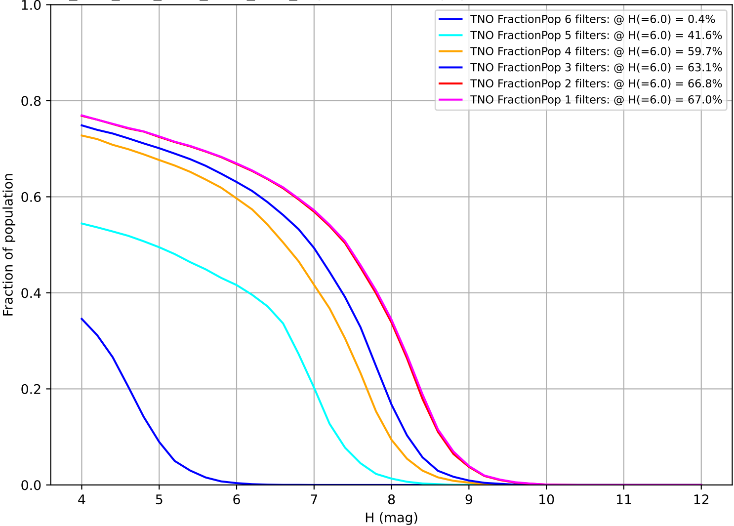
ddf_acor_sf10_lsf20_lsr50_v3.4_10yrs: Fraction of population with colors in X filters TNO
