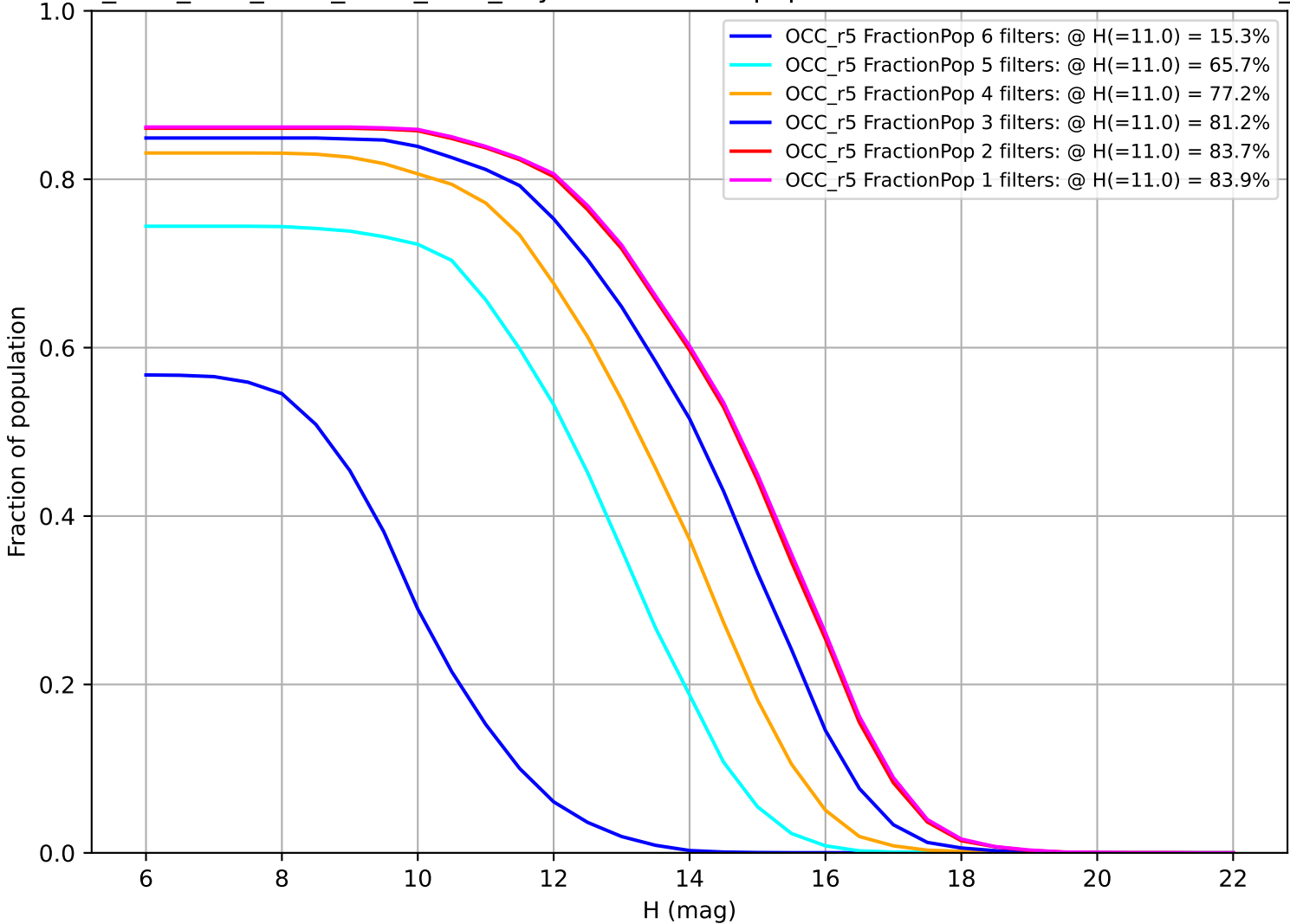
ddf_acor_sf10_lsf20_lsr50_v3.4_10yrs: Fraction of population with colors in X filters OCC_r5
