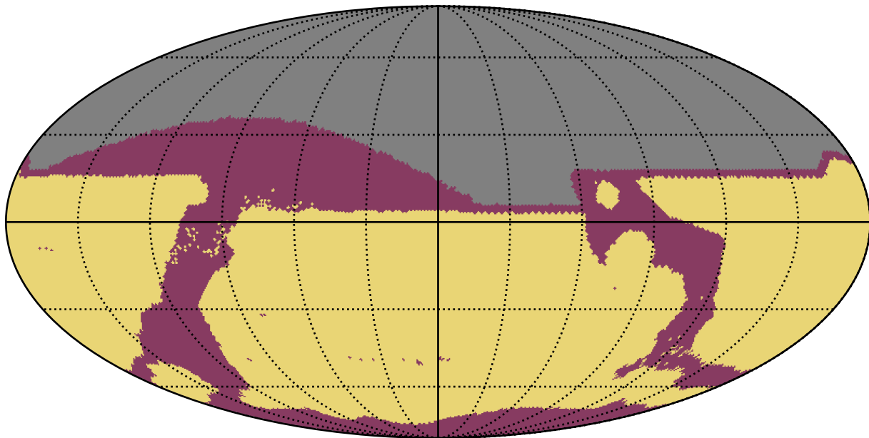
ddf_acor_sf10_lsf20_lsr50_v3.4_10yrs : RapidRevisits
