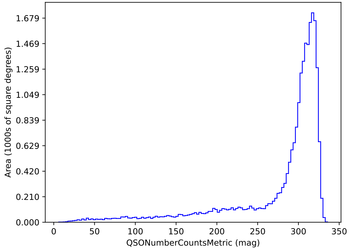
ddf_acor_sf10_lsf20_lsr50_v3.4_10yrs u band and non-DD: QSONumberCountsMetric
