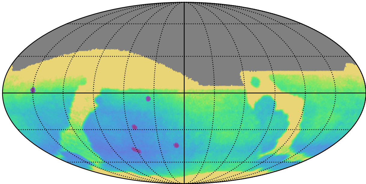
ddf_acor_sf10_lsf20_lsr50_v3.4_10yrs : Parallax Uncert @ 24.0
