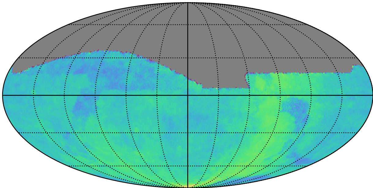
ddf_acor_sf10_lsf20_lsr50_v3.4_10yrs : Parallax Coverage @ 24.0
