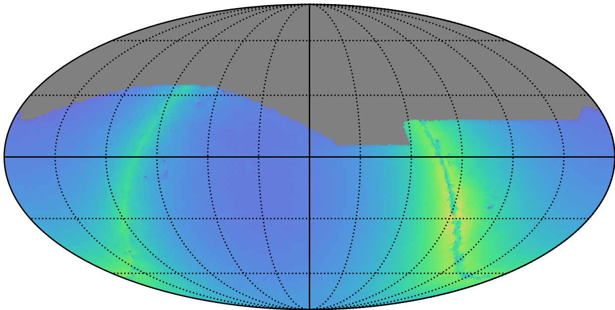
ddf_acor_sf10_lsf20_lsr50_v3.4_10yrs r: Nstars_no_crowding
