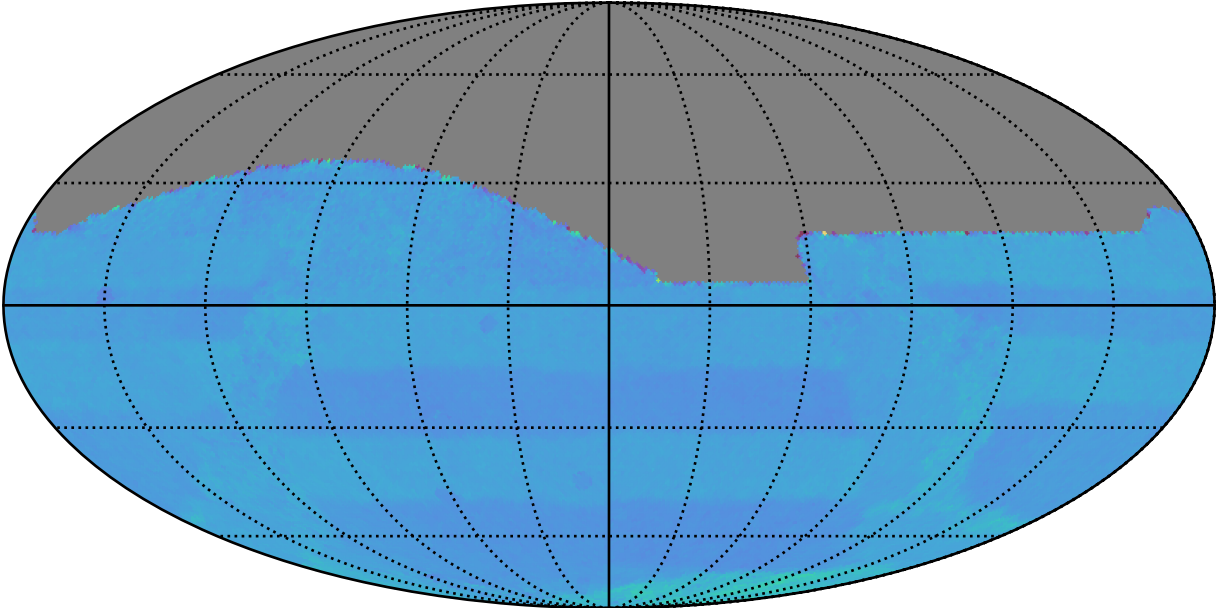
ddf_acor_sf10_lsf20_lsr50_v3.4_10yrs : Normalized Proper Motion Uncert @ 20.5
