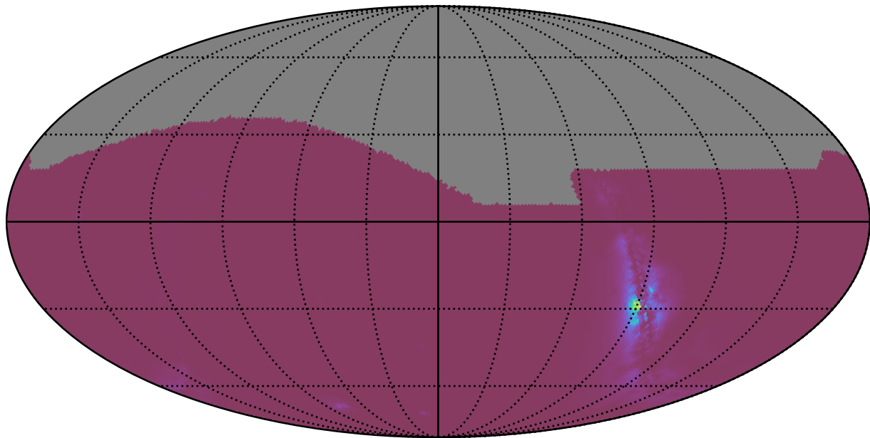
ddf_acor_sf10_lsf20_lsr50_v3.4_10yrs : NlcPoints
