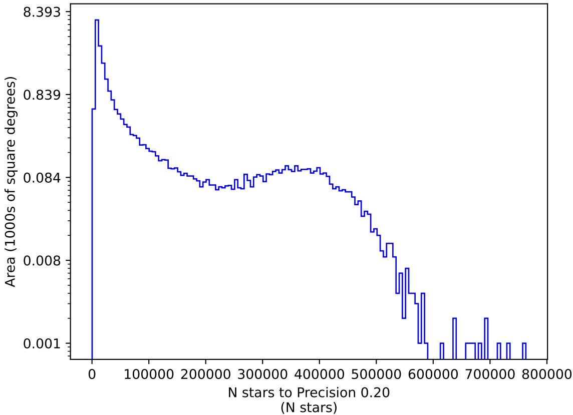
ddf_acor_sf10_lsf20_lsr50_v3.4_10yrs y: N stars to Precision 0.20
