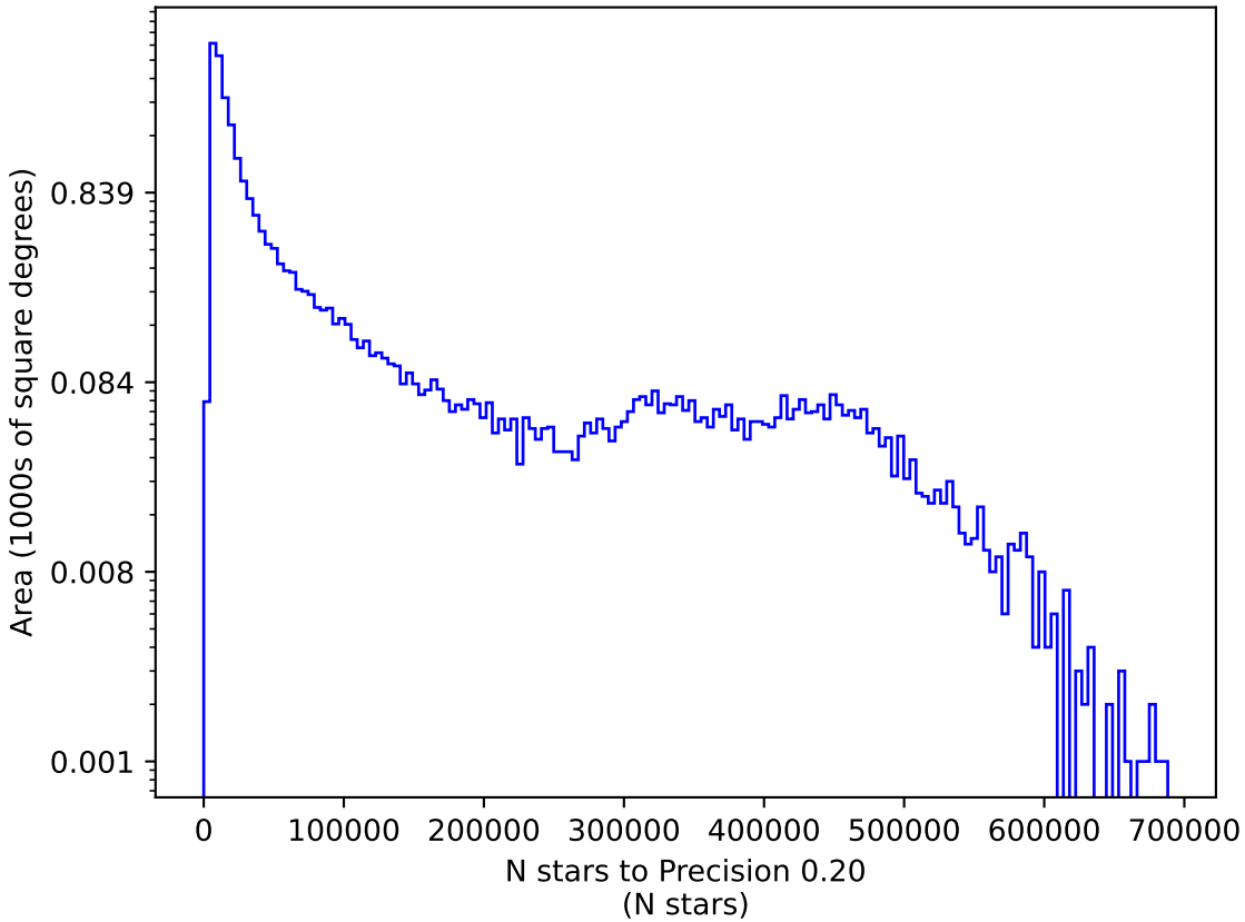
ddf_acor_sf10_lsf20_lsr50_v3.4_10yrs r: N stars to Precision 0.20
