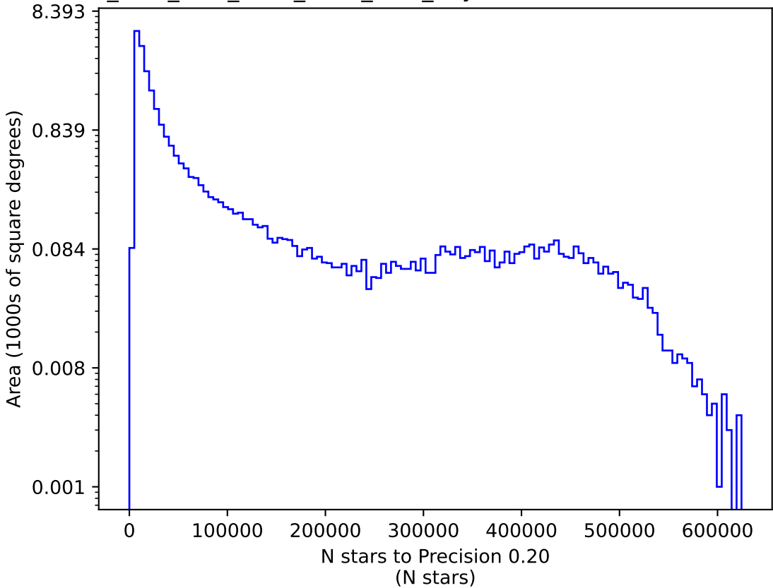
ddf_acor_sf10_lsf20_lsr50_v3.4_10yrs i: N stars to Precision 0.20
