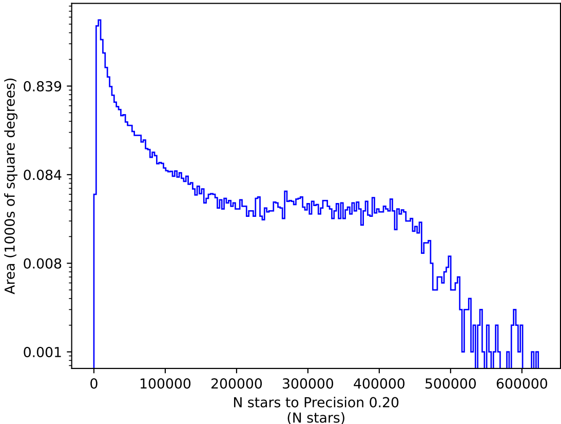
ddf_acor_sf10_lsf20_lsr50_v3.4_10yrs g: N stars to Precision 0.20
