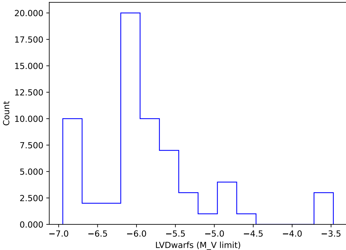
ddf_acor_sf10_lsf20_lsr50_v3.4_10yrs gi: LVDwarfs
