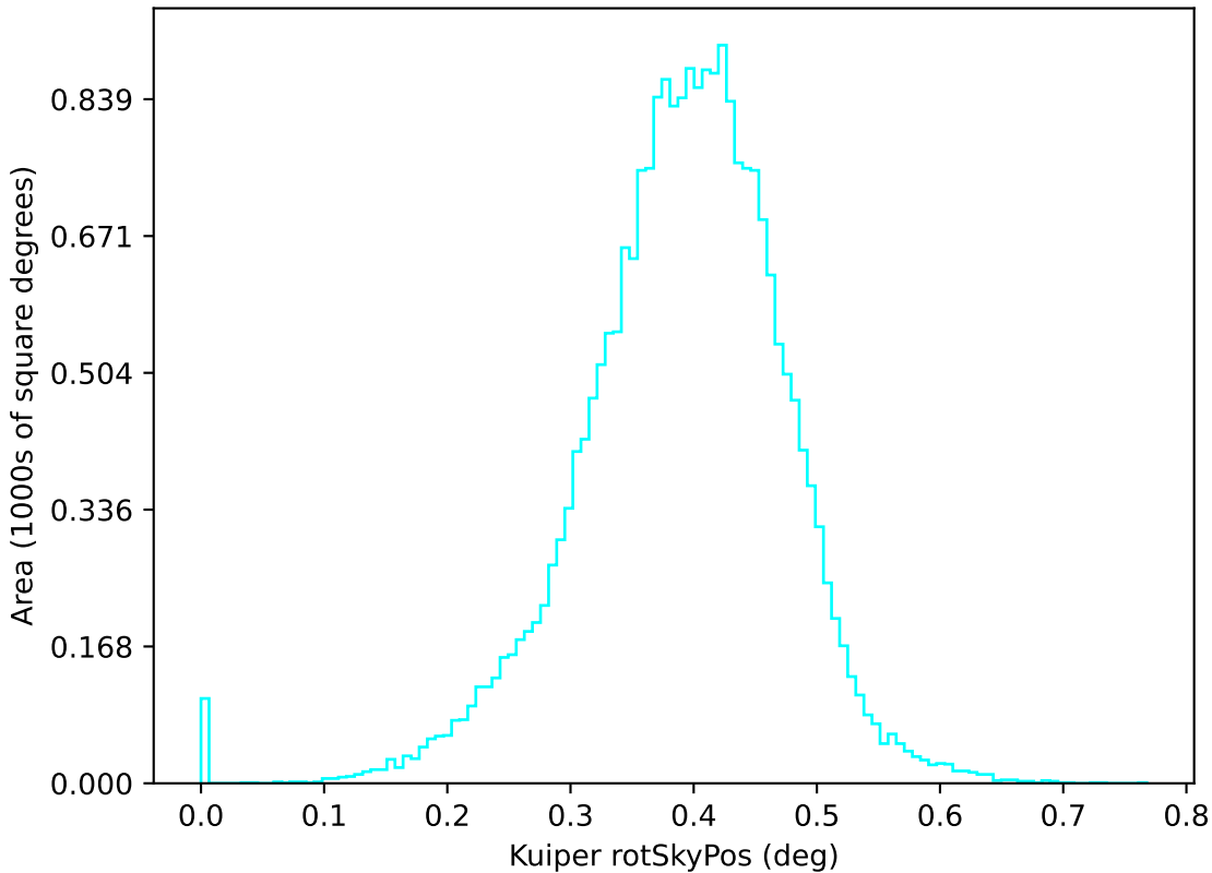
ddf_acor_sf10_ls20_lsr50_v3.4_10yrs u: Kuiper rotSkyPos
