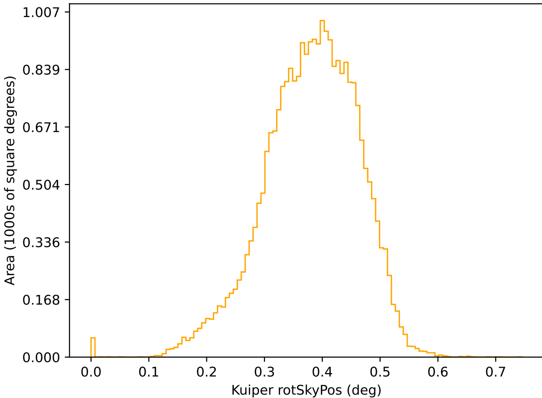
ddf_acor_sf10_lsfl20_lsr50_v3.4_10yrs r: Kuiper rotSkyPos
