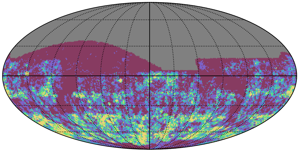
ddf_acor_sf10_lsf20_lsr50_v3.4_10yrs r band: Gaps_3hr
