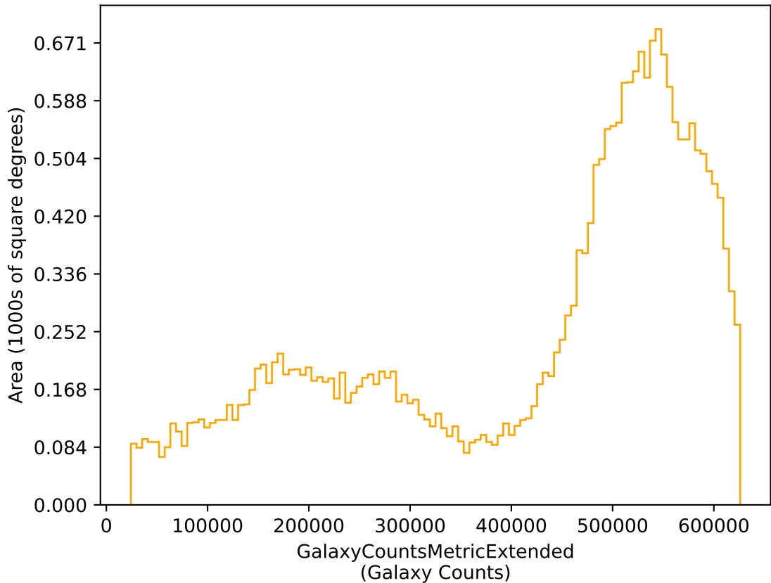
ddf_acor_sf10_lsf20_lsr50_v3.4_10yrs r: GalaxyCountsMetricExtended
