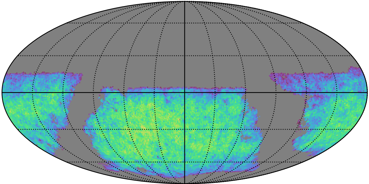
ddf_acor_sf10_lsf20_lsr50_v3.4_10yrs i band non-DD year 1: ExgalM5WithCuts
