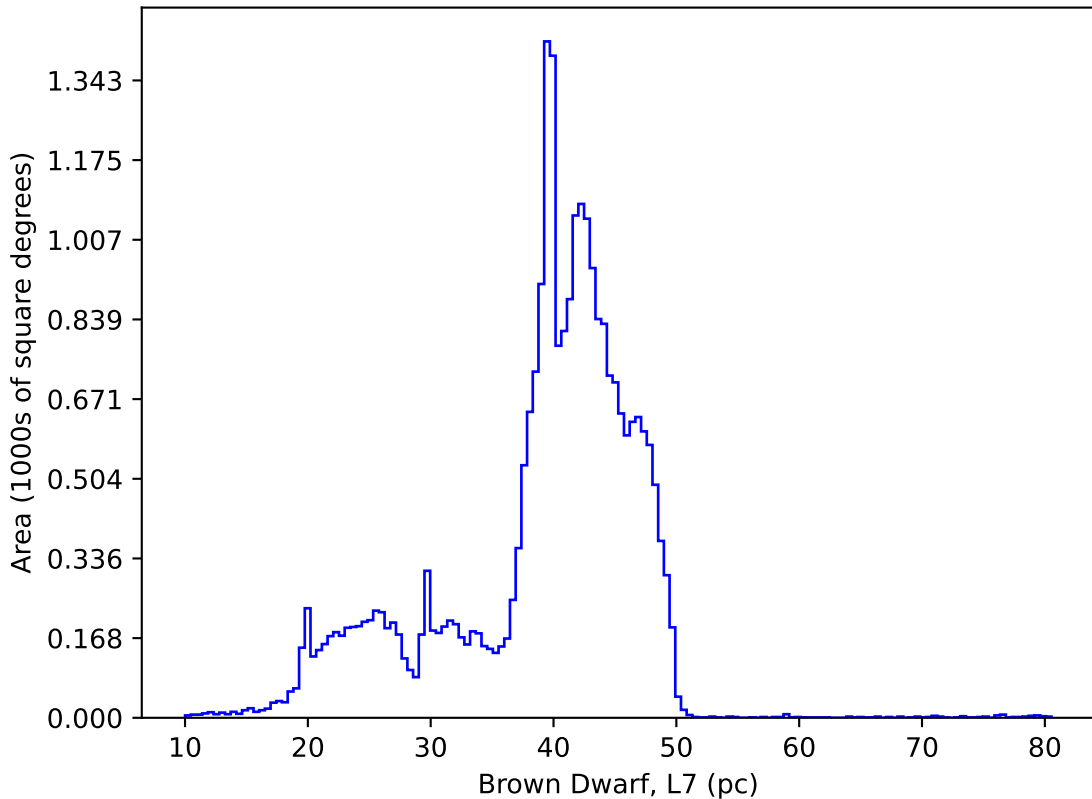
ddf_acor_sf10_lsf20_lsr50_v3.4_10yrs : Brown Dwarf, L7
