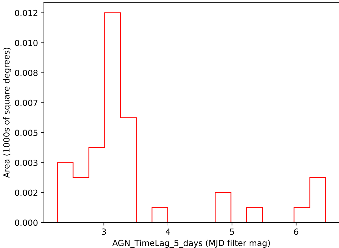
ddf_acor_sf10_ls20_lsr50_v3.4_10yrs i band: AGN_TimeLag_5_days
