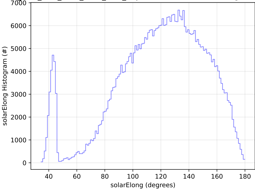
ddf_acor_sf10_lsf20_lsr50_v3.4_10yrs WFD z band: solarElong Histogram
