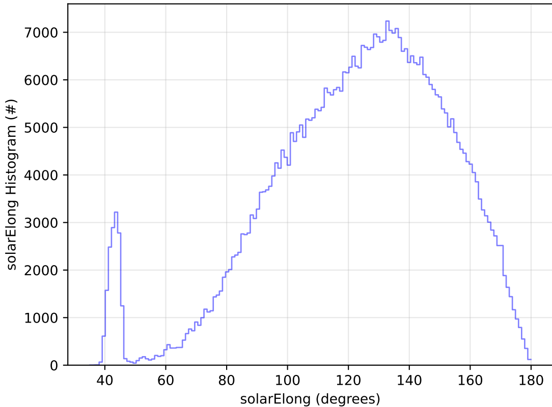
ddf_acor_sf10_lsf20_lsr50_v3.4_10yrs WFD r band: solarElong Histogram
