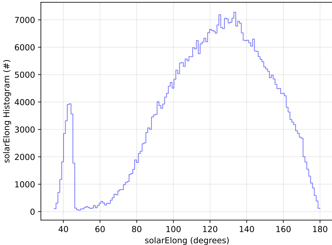
ddf_acor_sf10_lsf20_lsr50_v3.4_10yrs WFD i band: solarElong Histogram
