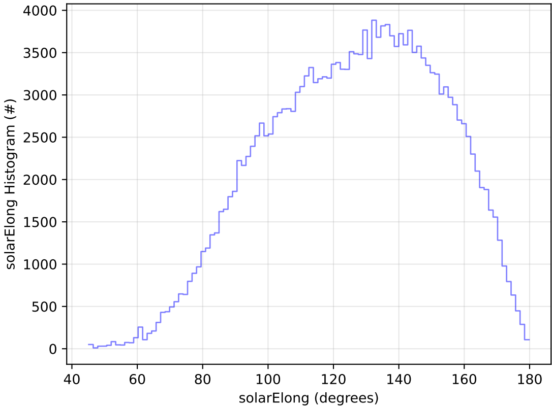
ddf_acor_sf10_lsf20_lsr50_v3.4_10yrs WFD g band: solarElong Histogram
