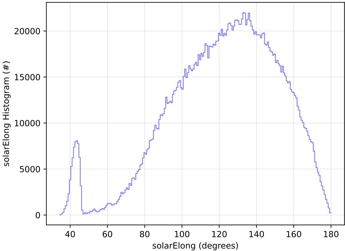
ddf_acor_sf10_lsf20_lsr50_v3.4_10yrs WFD all bands: solarElong Histogram
