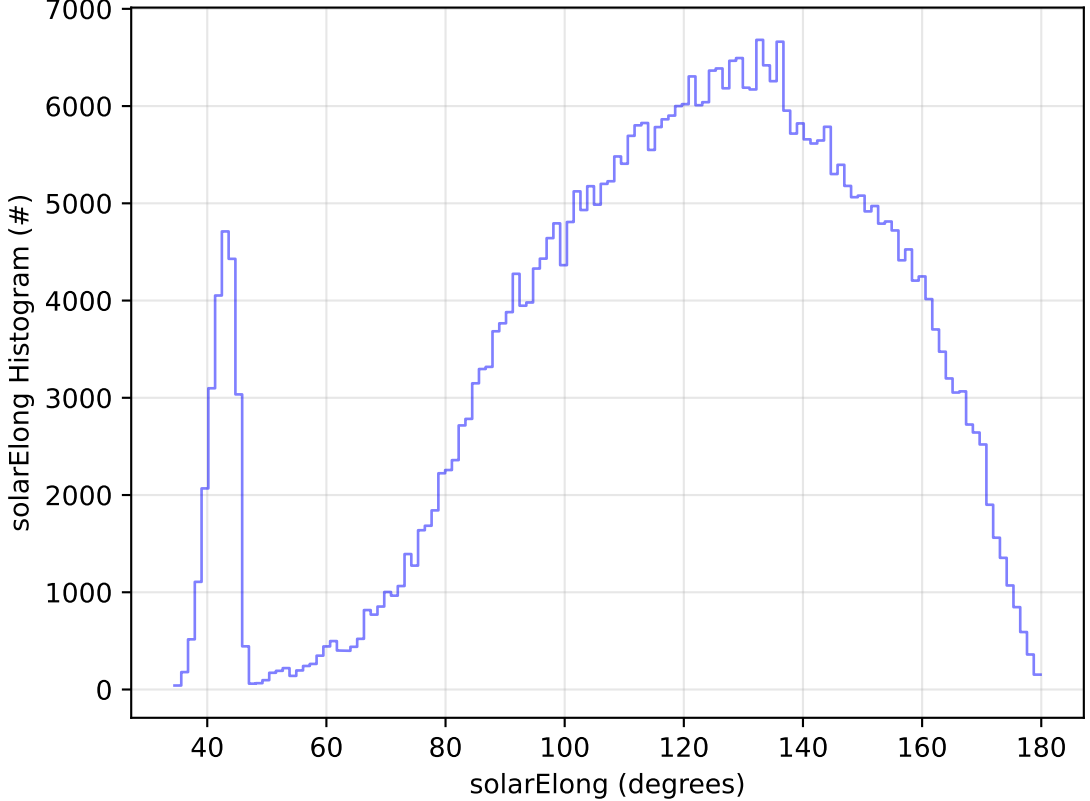
ddf_acor_sf10_lsf20_lsr50_v3.4_10yrs All sky z band: solarElong Histogram
