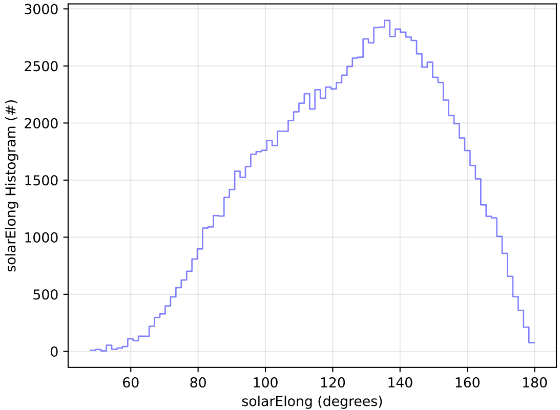
ddf_acor_sf10_lsf20_lsr50_v3.4_10yrs All sky u band: solarElong Histogram
