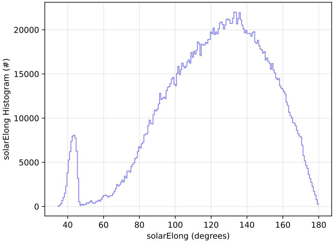
ddf_acor_sf10_lsf20_lsr50_v3.4_10yrs All sky all bands: solarElong Histogram
