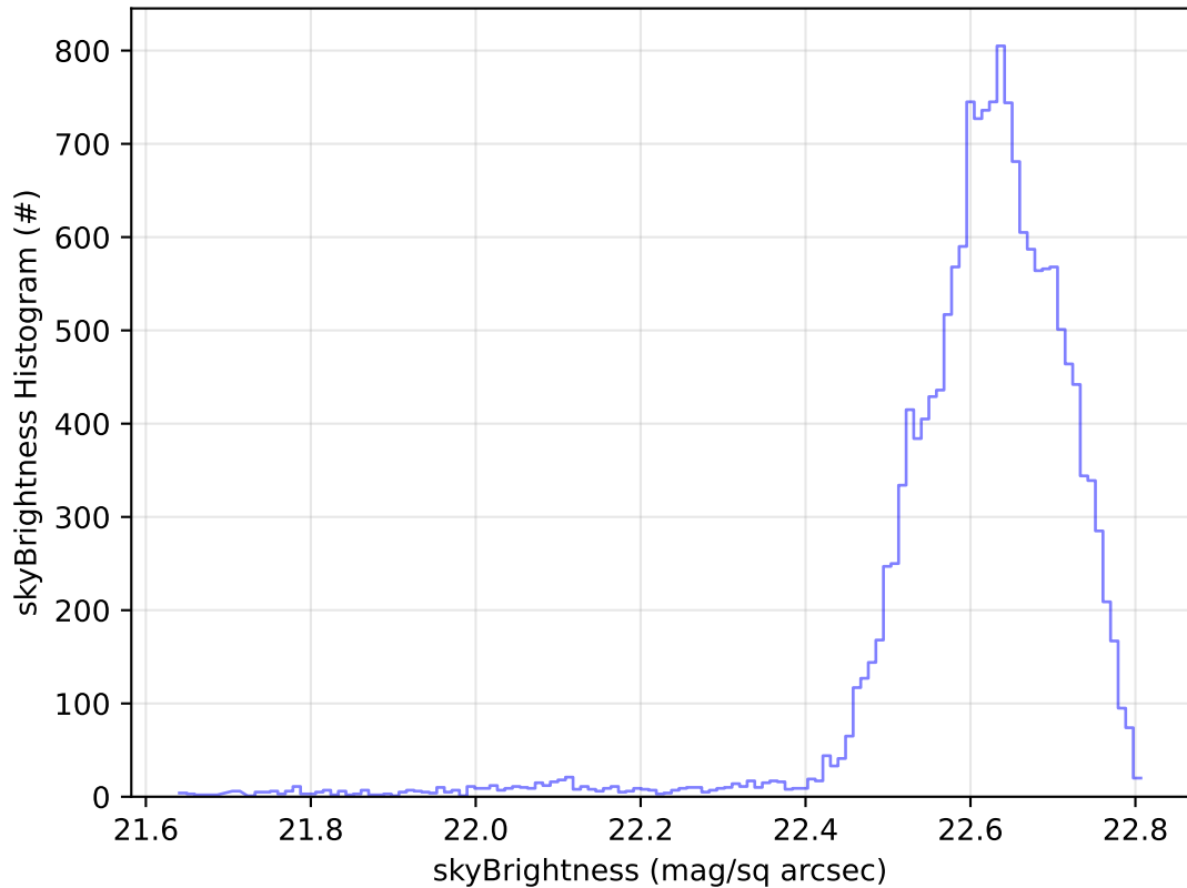
ddf_acor_sf10_lsf20_lsr50_v3.4_10yrs Yr 1 u band: skyBrightness Histogram
