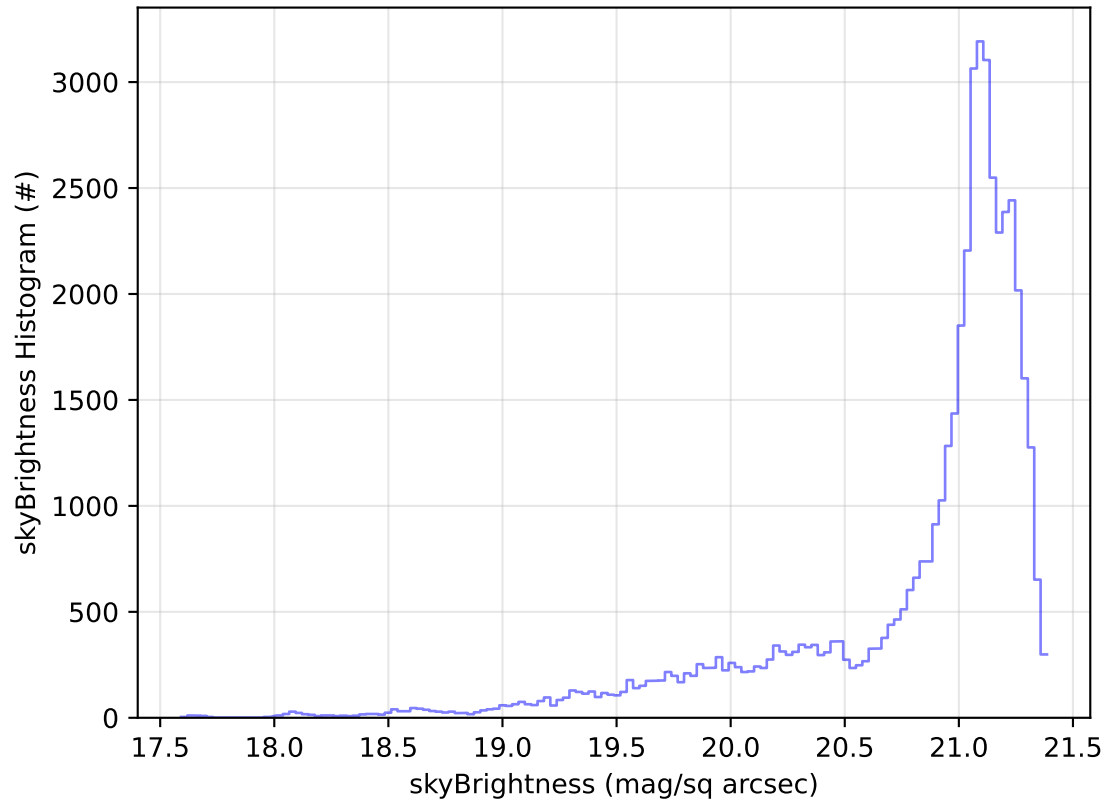
ddf_acor_sf10_lsf20_lsr50_v3.4_10yrs Yr 1 r band: skyBrightness Histogram
