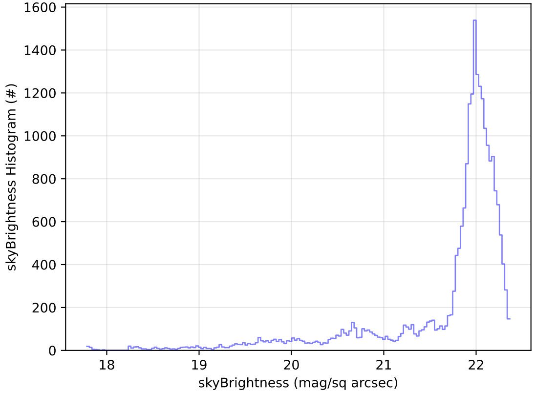
ddf_acor_sf10_lsf20_lsr50_v3.4_10yrs Yr 1 g band: skyBrightness Histogram
