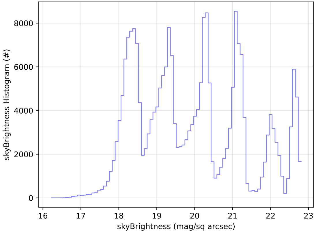
ddf_acor_sf10_lsf20_lsr50_v3.4_10yrs Yr 1 all bands: skyBrightness Histogram
