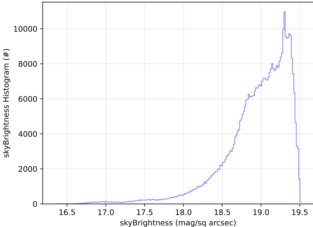
ddf_acor_sf10_lsf20_lsr50_v3.4_10yrs WFD z band: skyBrightness Histogram
