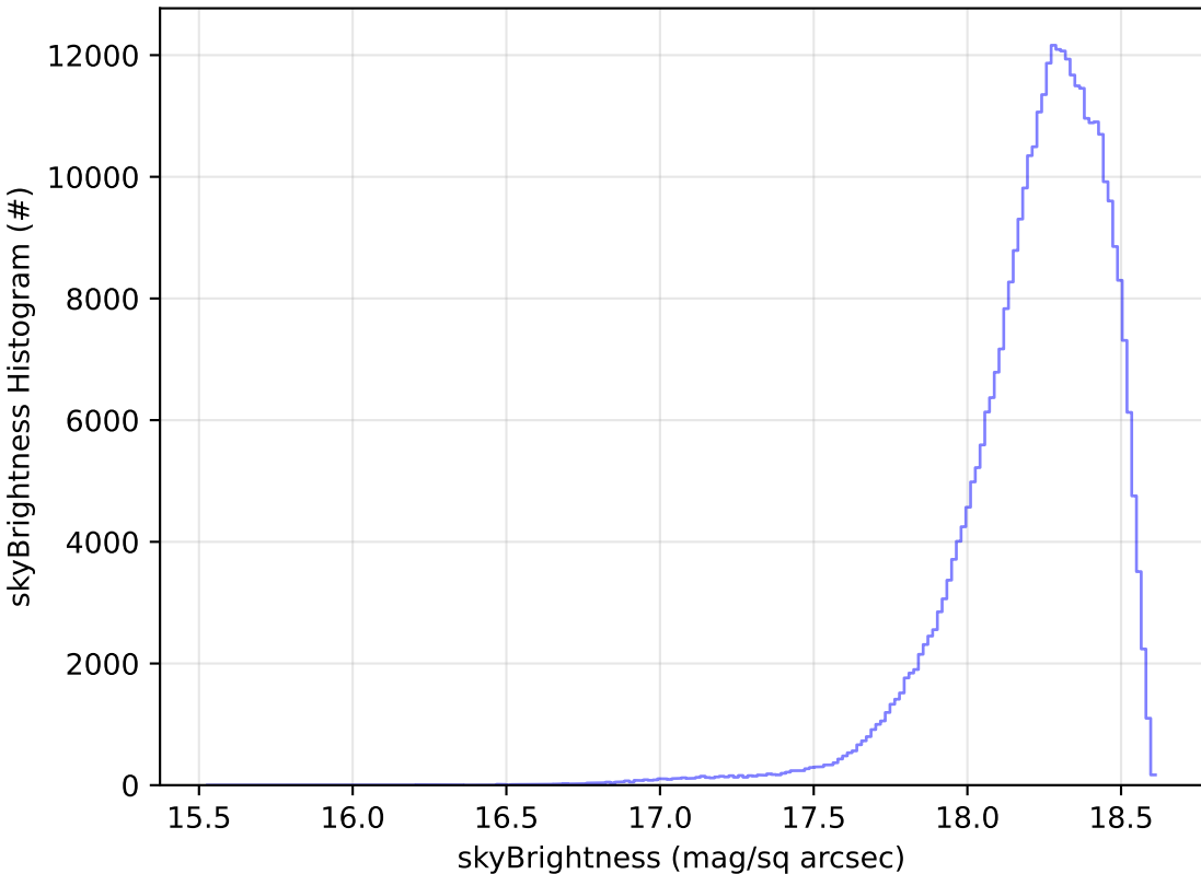
ddf_acor_sf10_lsf20_lsr50_v3.4_10yrs WFD y band: skyBrightness Histogram
