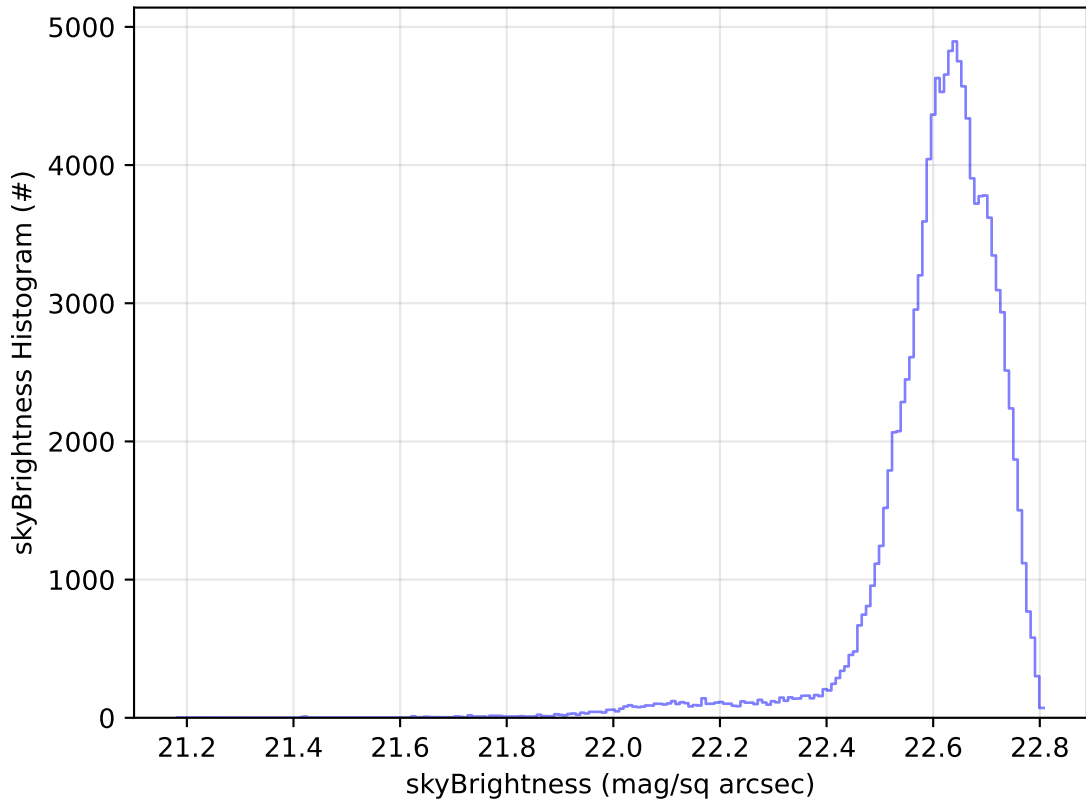
ddf_acor_sf10_lsf20_lsr50_v3.4_10yrs WFD u band: skyBrightness Histogram
