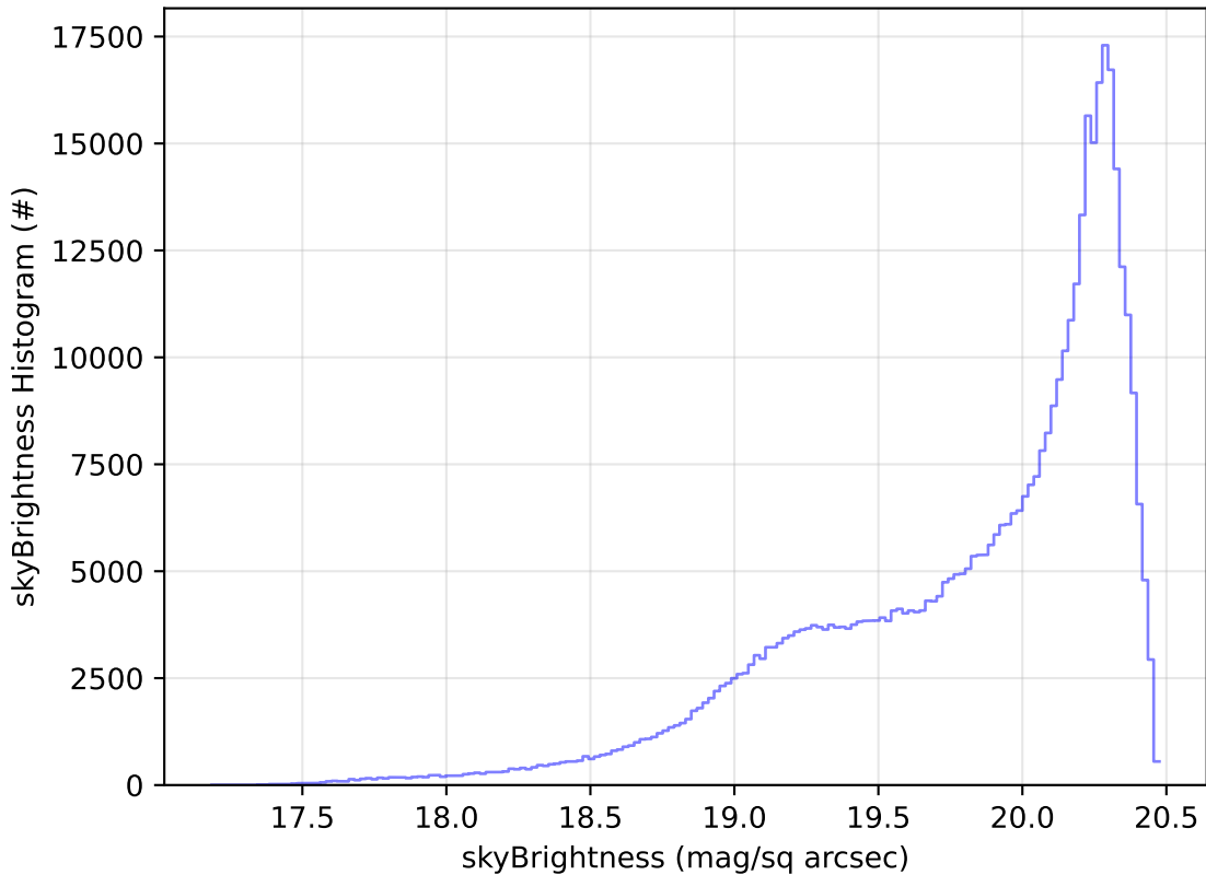
ddf_acor_sf10_lsf20_lsr50_v3.4_10yrs WFD i band: skyBrightness Histogram
