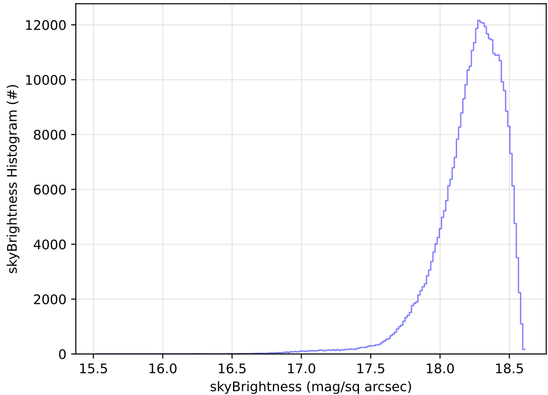
ddf_acor_sf10_lsf20_lsr50_v3.4_10yrs All sky y band: skyBrightness Histogram
