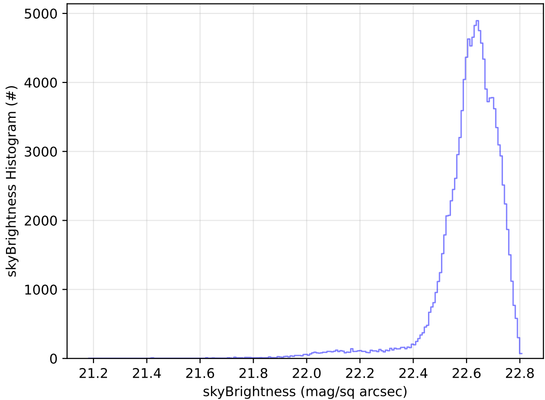
ddf_acor_sf10_lsf20_lsr50_v3.4_10yrs All sky u band: skyBrightness Histogram
