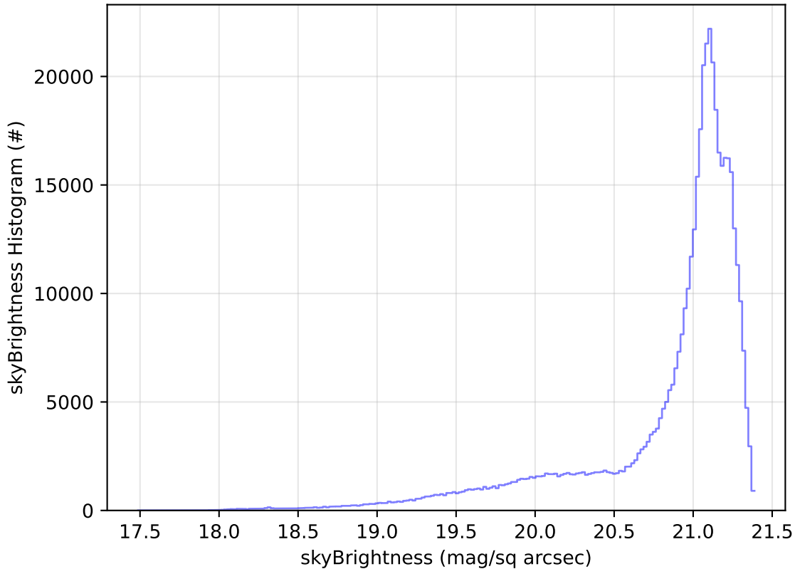
ddf_acor_sf10_lsf20_lsr50_v3.4_10yrs All sky r band: skyBrightness Histogram
