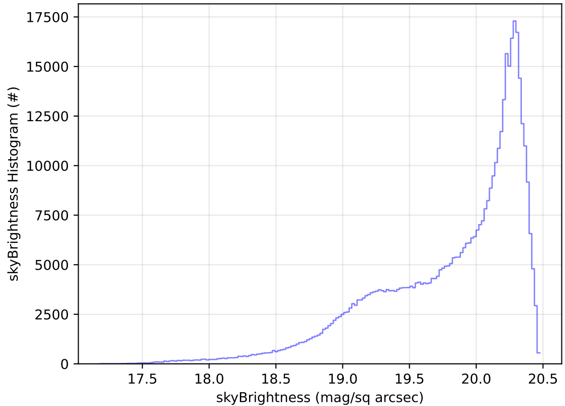
ddf_acor_sf10_lsf20_lsr50_v3.4_10yrs All sky i band: skyBrightness Histogram
