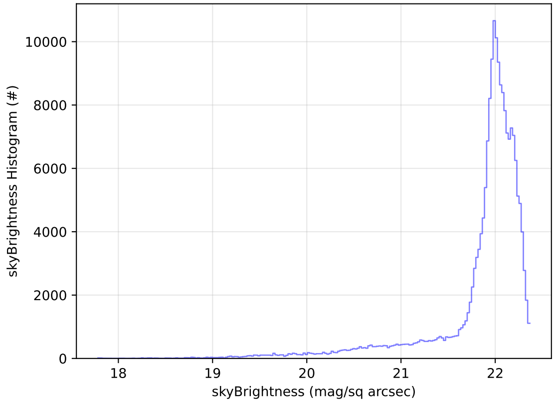
ddf_acor_sf10_lsf20_lsr50_v3.4_10yrs All sky g band: skyBrightness Histogram
